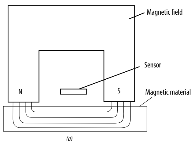
Figure 2. Magnetic leakage field from the magnetic material without (a) and with (b) a defect.
